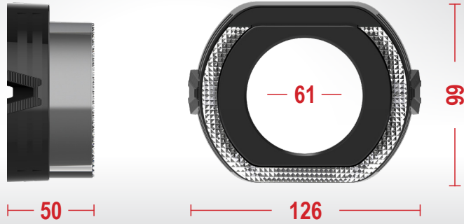
W9-U25 2.5inch
