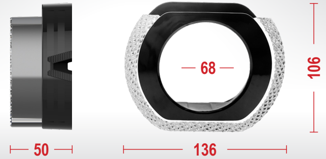
W9-U30 3.0inch
