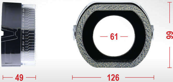
W9-O25 2.5inch
