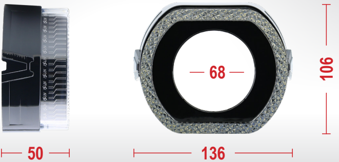
W9-O30 3.0inch
